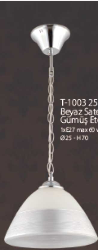
T-1003 25 Beyaz Saten Bal Etek 1xE27 max 60 w Ø 25 - H 70
